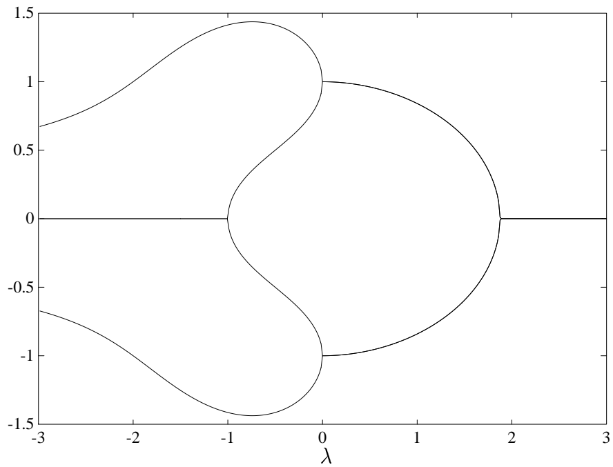
Figure 3: Imaginary parts of the eigenvalues in example b) against the bifurcation parameter \lambda . The sequence splitting at 0 \rightarrow splitting at \pm i can be observed as \lambda is varied. The last eigenvalue bifurcation is related to splitting off the real axis , but this does not correspond to a dynamic bifurcation.
