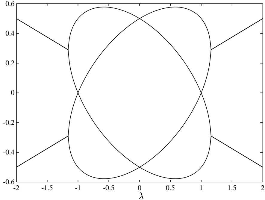
Figure 4: Imaginary parts of all four eigenvalues in example d) against the angular velocity \lambda . The sequence indefinite splitting \rightarrow passing at 0 \rightarrow definite passing \rightarrow passing at 0 \rightarrow indefinite splitting can be observed as \lambda is varied.
