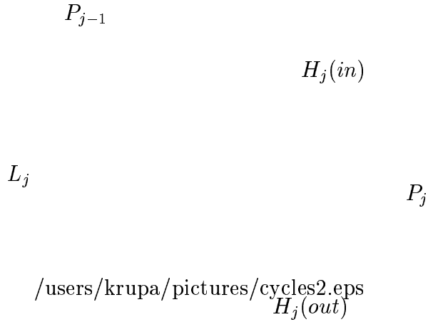
Figure 2: The cross-sections H_j^{(in)} and H_j^{(out)}
