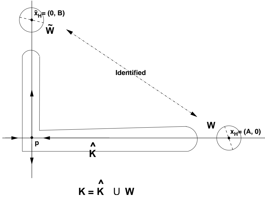
FIGURE 1. Basic local setup near the \Phi -orbit of x_H
